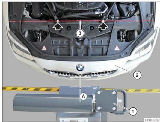
Fig. 16: Positioning Headlight Adjustment Device Courtesy of BMW OF NORTH AMERICA, INC.
